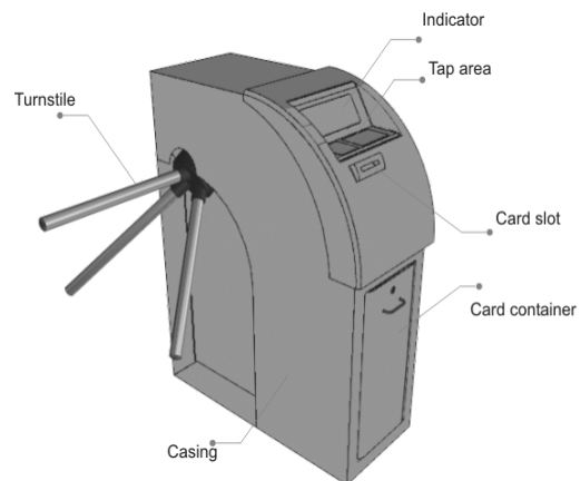
Figure 14. Gate Access
